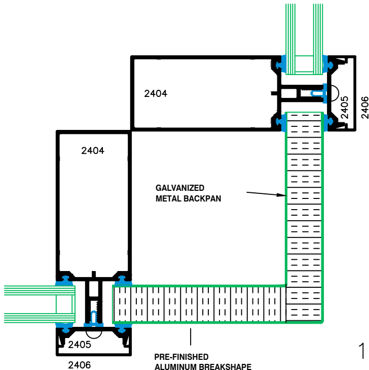
90° BREAKSHAPE CORNER
