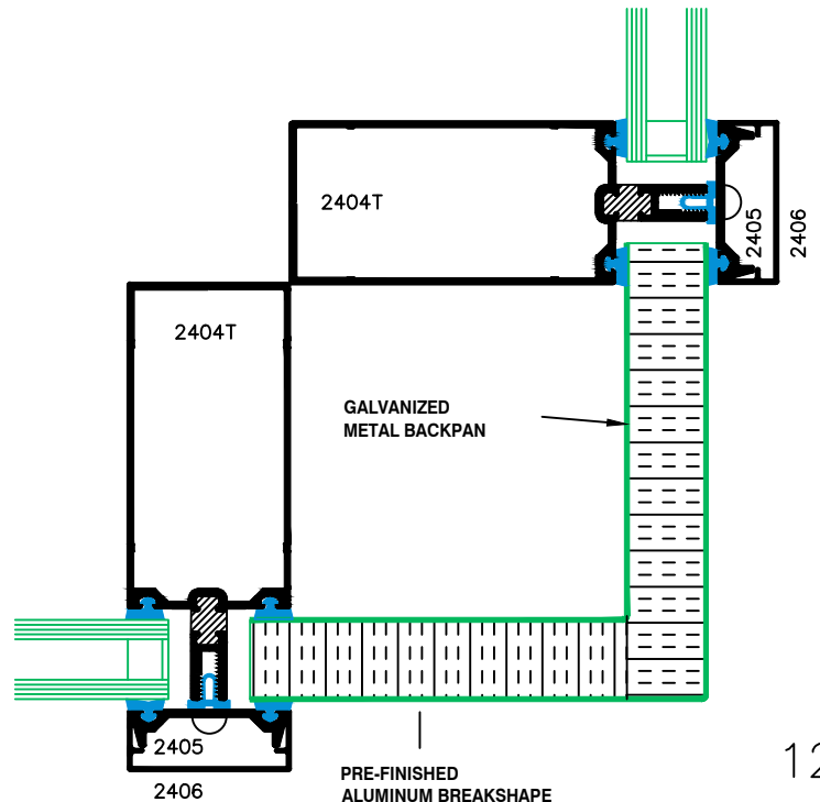
90° BREAKSHAPE CORNER
