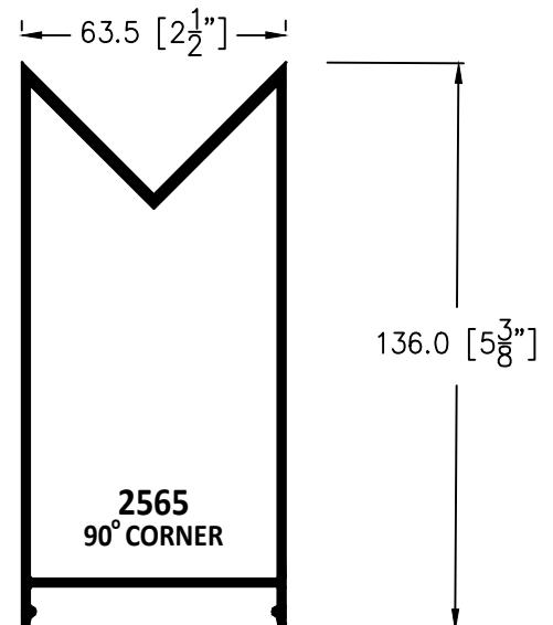
EXTENSION CAP FOR 5 1/4" BACK
