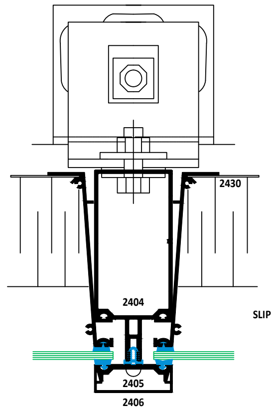
PLAN DETAILS
