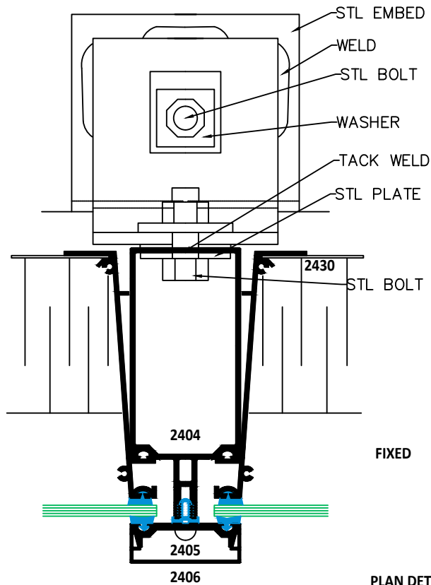
PLAN DETAILS
