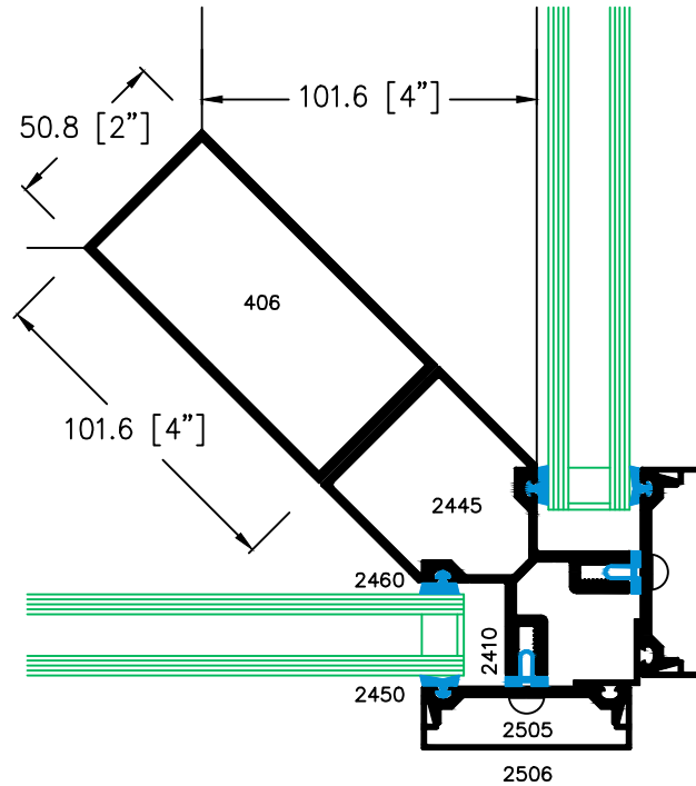
90° CAPTURED CORNER
