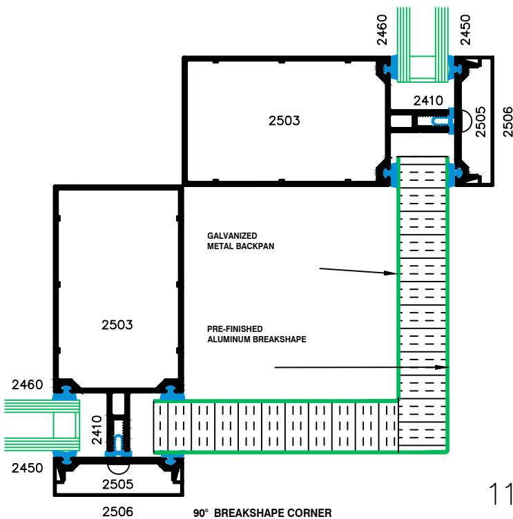
90° BREAKSHAPE CORNER
