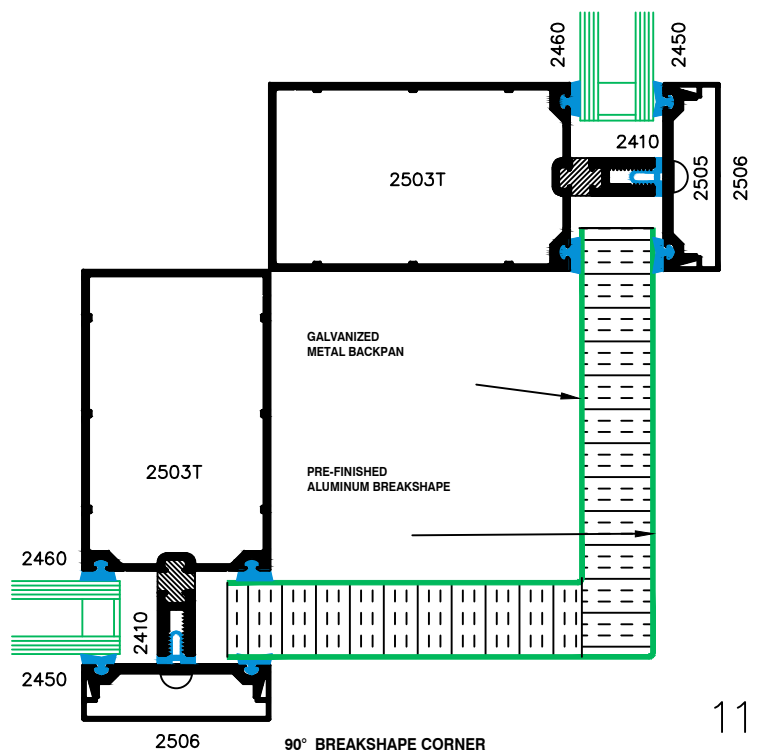
90° BREAKSHAPE CORNER
