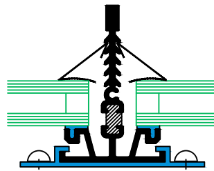
2 T/B RAFTER DOUBLE GLAZING
