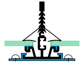
2 RAFTER SINGLE GLAZING
