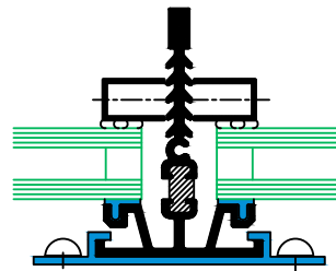
2 GLAZING WITH C-SHAPE
