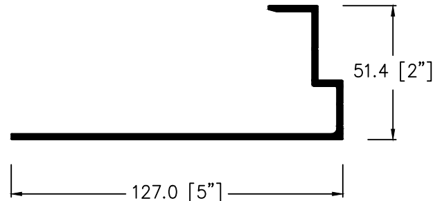
3010 SILL - CONTINUOUS SHOE
