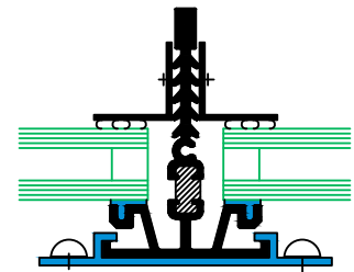
2 GLAZING WITH L-SHAPE
