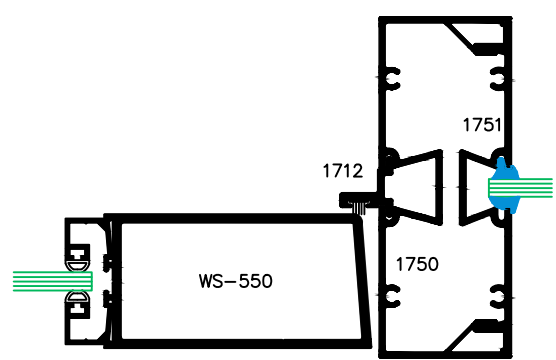
OFFSET HUNG
