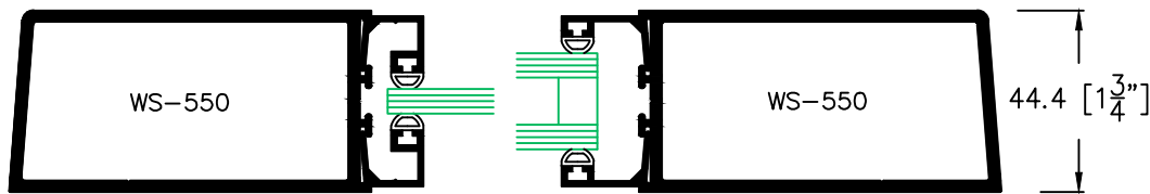
SINGLE GLAZED
