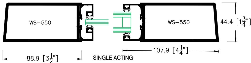
SINGLE GLAZED
