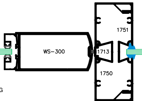
CENTER HUNG
