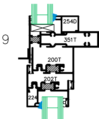
OPEN-OUT VENT 200T SERIES
