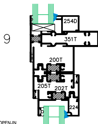
OPEN-IN VENT 200T SERIES
