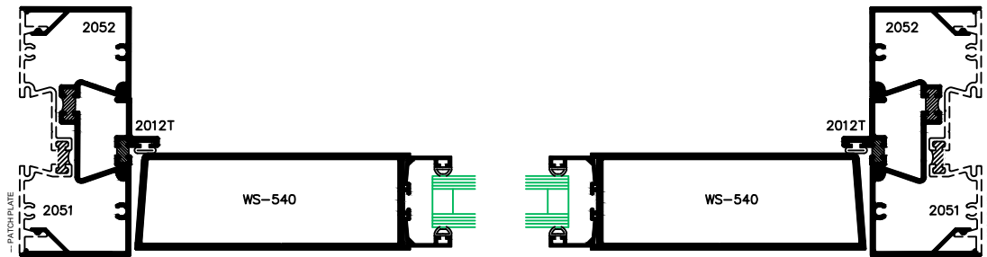
OFFSET HUNG
